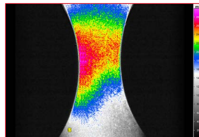
Thermal Stress Analysis with Lock-in Thermography
