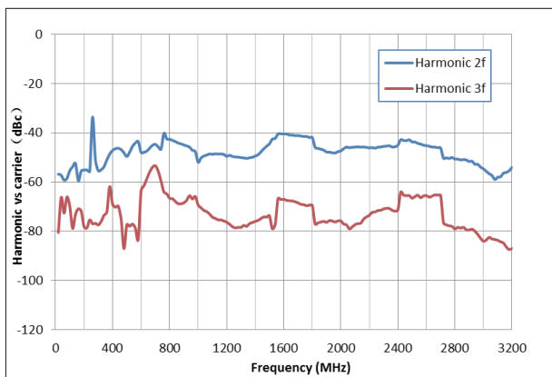
Measured harmonics versus carrier frequency at level ≤ +13 dBm
