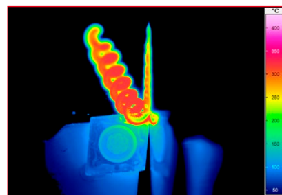
Machining process with a tool bit
