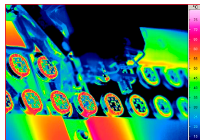
Bonding of sensors
